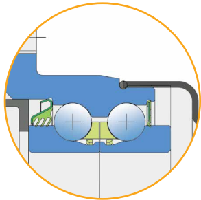
Plastic cover + 3-lip seal/RS seal + Threaded metal cap
