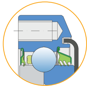
S seal/3-lip seal + Metal shield
