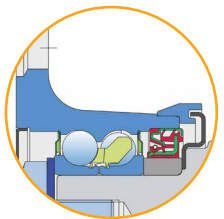
Sheet metal shield + S seal/S seal + Dirtblock seal + Metal shield
