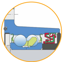
O-ring + Sheet metal shield + S seal/S seal + Dirtblock seal + Forged cover plate
