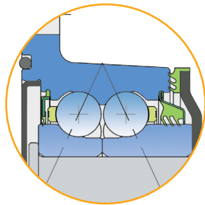
Sheet metal shield + RS seal/3-lip seal + Front 3-lip seal + Metal protective cover
