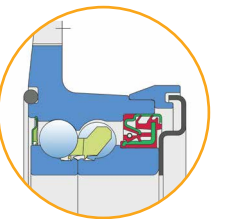
O-ring + S seal/Dirtblock seal + Metal shield
