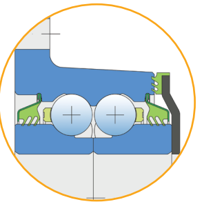
3-lip seal/3-lip seal + Front 3-lip seal + Metal protective cover
