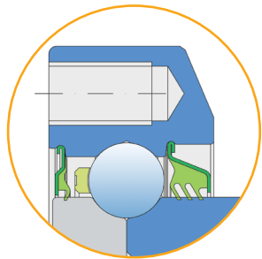
S seal/3-lip seal
